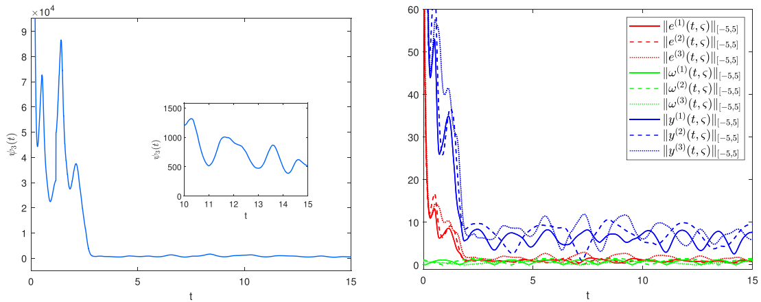
Fig. 6. Evolution of function \psi_3(t) and the error e_i^k(t, \zeta) in Case III.
